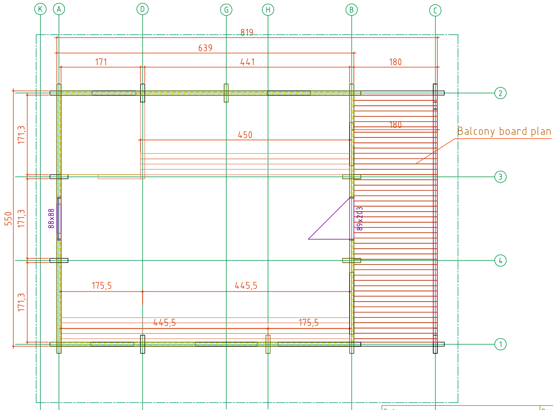
First floor board. Plan
