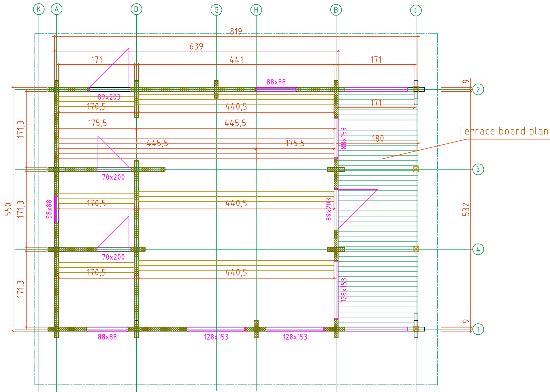
Ground floor boards. Plan
