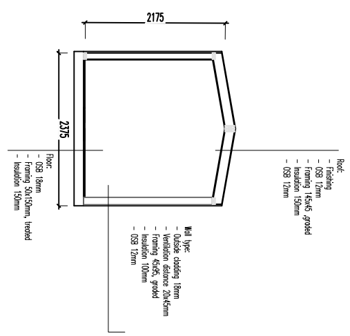
Section 1-1 1:50
