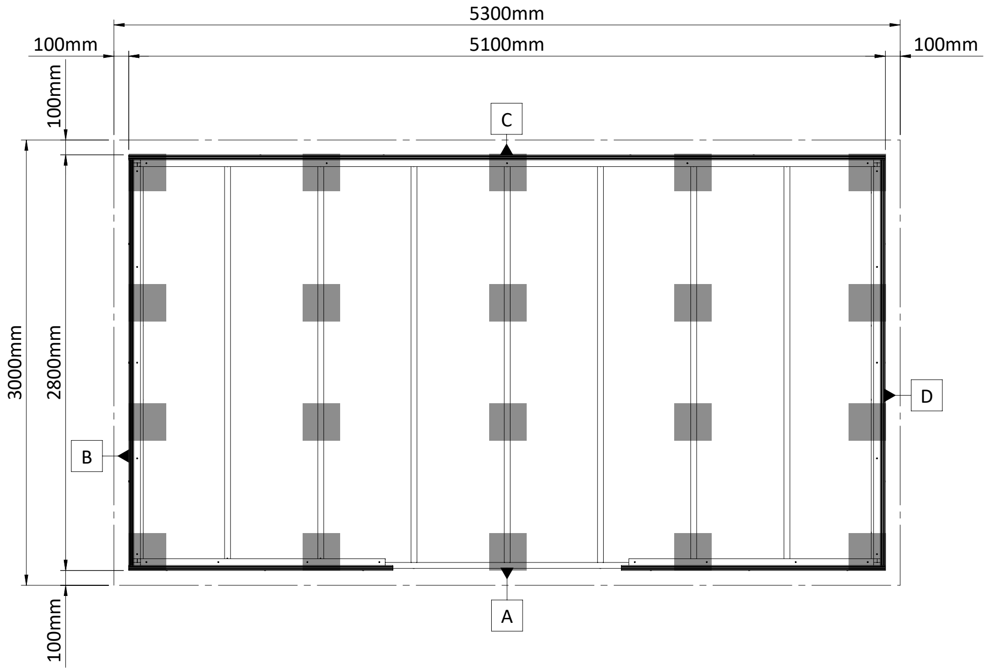
PLINTPLAN / FOUNDATION PLAN / BETONBLOCK / PLAN DE FONDATIONS
